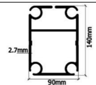
Eave purlin
